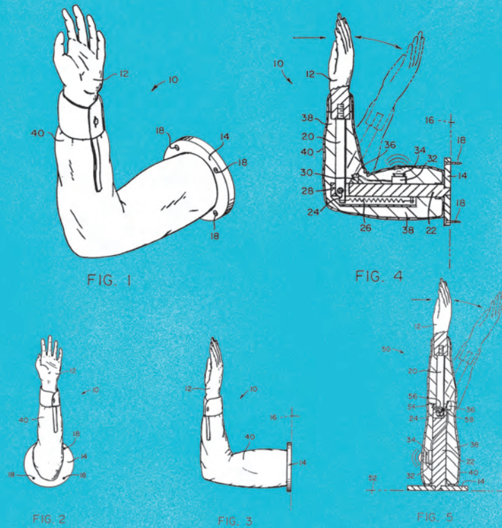
High Five Machine - US Patent Office - 07. Dec. 1993
